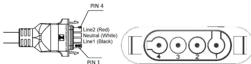
Figure 24: Pin configuration for AC cables.
